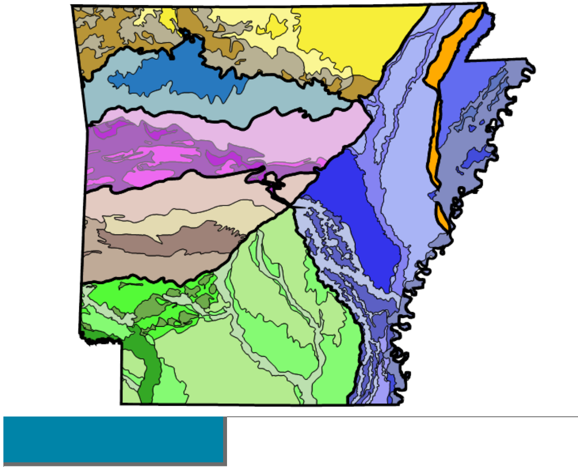
Figure II-2: Arkansas's Ecoregions
