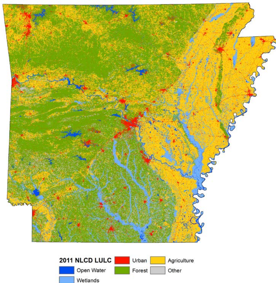
Figure II-1: Land Use
